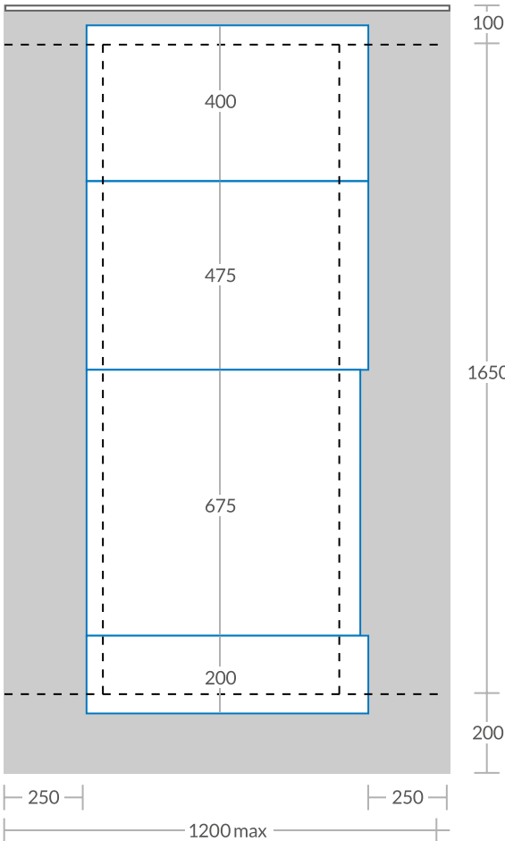
Urinal Panel System
