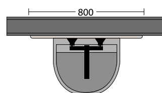
Standard Pre Assembled Recessed Unit
